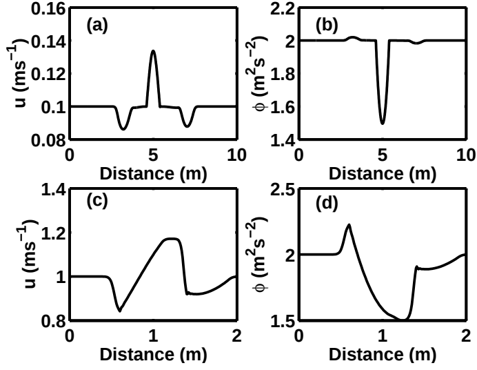
Figure 1: Initial conditions at time t = 0 . The plots show (a) u and (b) \phi for Case I and (c) u and (d) \phi for Case II.
