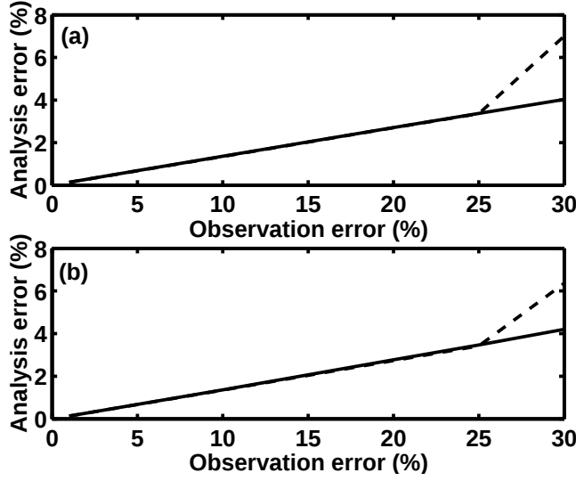
Figure 9: Case II: Plot of percentage analysis error at the centre of the time window, relative to the norm of the true solution, against level of observational noise, for (a) u field and (b) \phi field. The solid line indicates the assimilation using the TLM and the dashed line that using the PFM.
