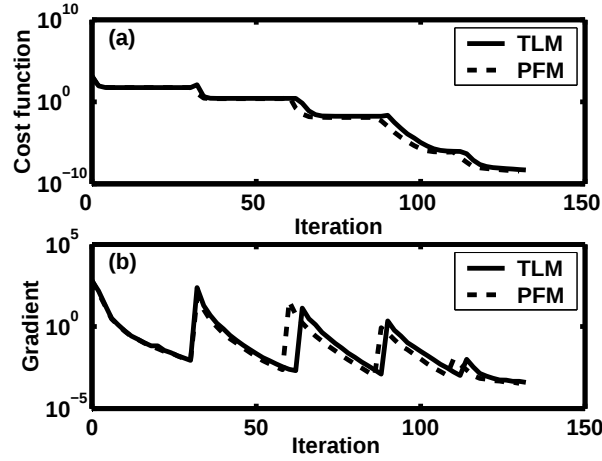
Figure 3: Case I: Convergence of (a) cost function and (b) gradient for tangent linear model (solid line) and perturbation forecast model (dashed line).
