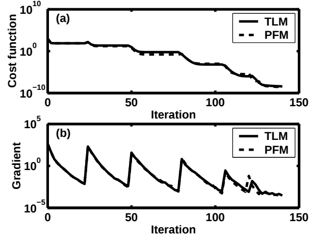
Figure 4: Case II: Convergence of (a) cost function and (b) gradient for tangent linear model (solid line) and perturbation forecast model (dashed line).
