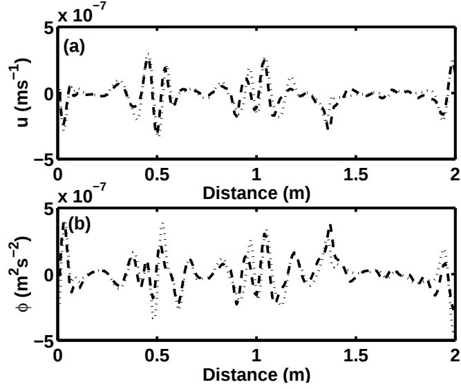
Figure 6: As for Figure 5, for Case II.
