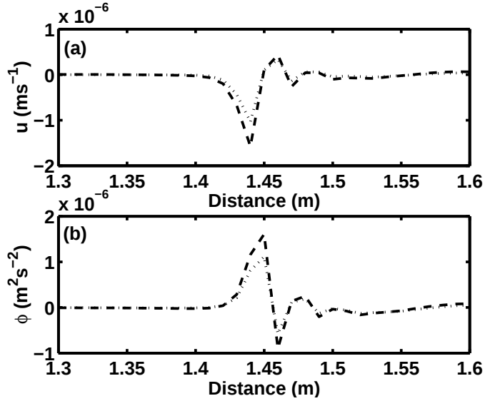
Figure 7: Case II: Error in the forecast around the shock position after 100 time steps for (a) u and (b) \phi . The dotted line is for the assimilation using the TLM and the dashed line for that using the PFM.
