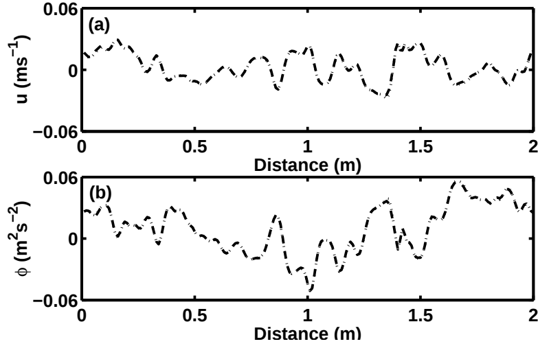
Figure 8: Case II: Analysis errors at the centre of the time window for (a) u field and (b) \phi field when noise is included on the observations. The dotted line indicates the assimilation using the TLM and the dashed line that using the PFM.
