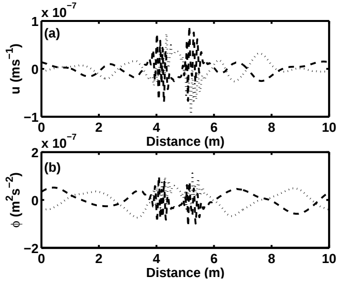
Figure 5: Case I: Analysis errors at the centre of the time window for (a) u field and (b) \phi field, with the dotted line indicating the assimilation using the TLM and the dashed line using the PFM.
