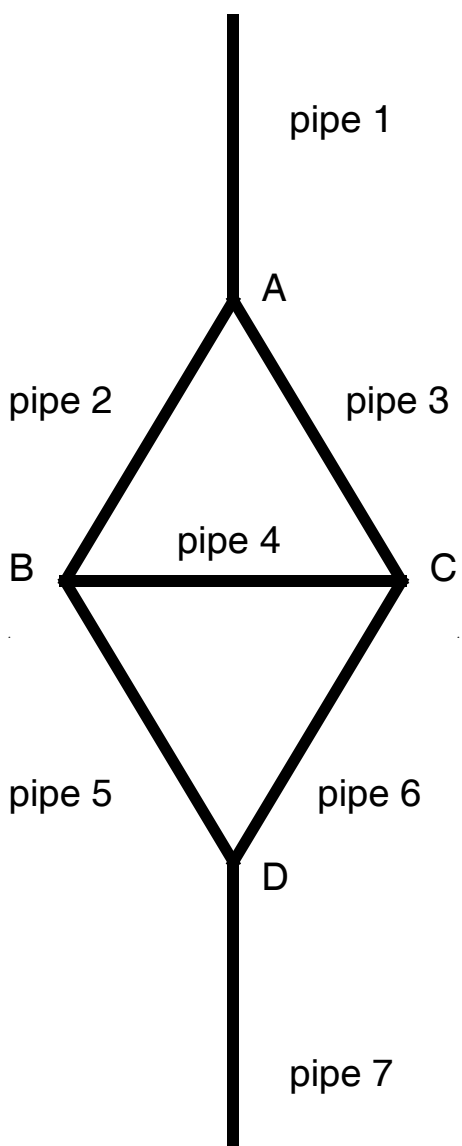
Figure 18: Looped network.
