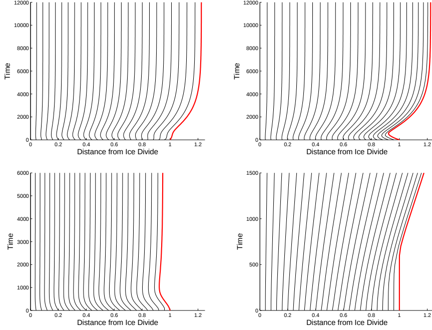
Figure 3: Evolution of the mesh nodes over time, including the boundary point (red) representing the glacier front.
