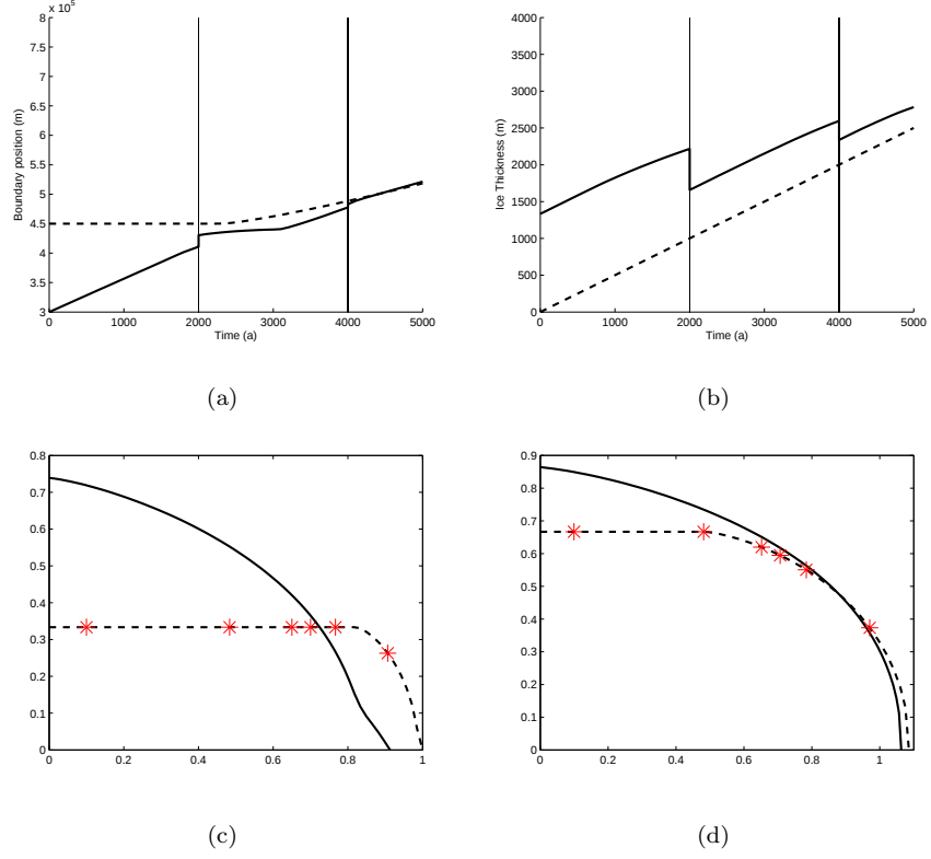
Figure 9: When less observations are available the convergence to the truth is slower
