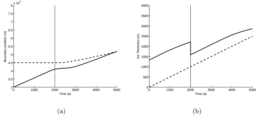
Figure 6: Effect of data assimilation on two key features, (a) Position of the moving boundary, and (b) Ice thickness at the divide. Solid lines represent the prediction, dashed lines denote the truth.
