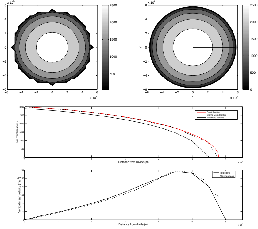
Figure 4: a) 2D results from one of the fixed grid EISMINT experiments. b) Moving mesh flowline radial model converted to 2D. c) Ice thickness profile at steady state showing the exact (red), moving mesh (dash) and fixed grid (solid) solutions. d) Diffusive velocity at steady state showing moving mesh (dash) and fixed grid (solid) solutions.
