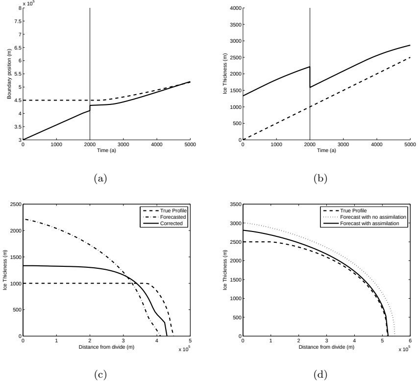
Figure 7: The numerical domain is corrected as well as the ice thickness by augmenting the data assimilation acheme.
