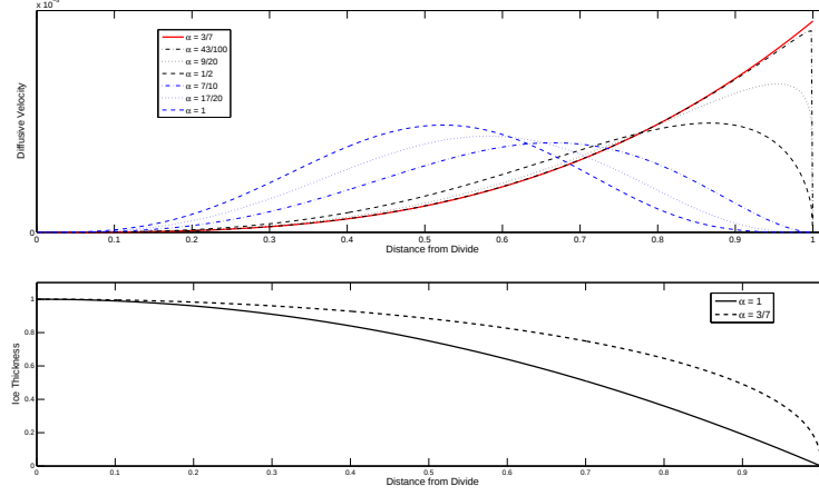
Figure 1: (a) Diffusive velocity. When \alpha = 3/7 (red line) the boundary velocity is finite whereas all other values have a zero boundary velocity. (b) Ice thickness profiles for \alpha = 1 (solid) and \alpha = 3/7 (dashed). Notice the infinite gradient at the boundary when \alpha \rightarrow 3/7 .
