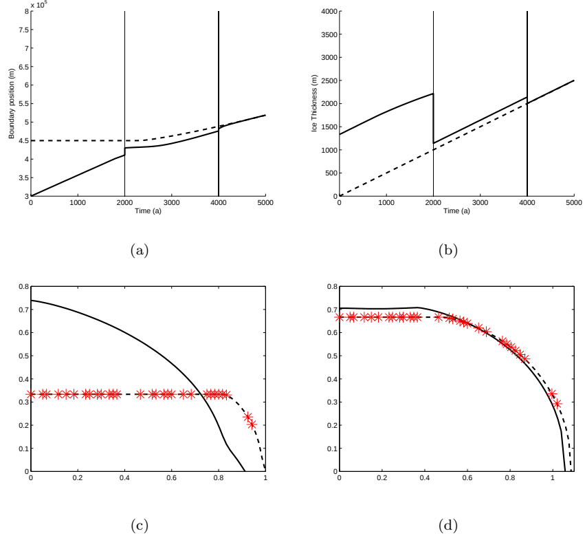
Figure 8: Taking lots of observations causes the forecast to converge towards the truth at a fast rate
