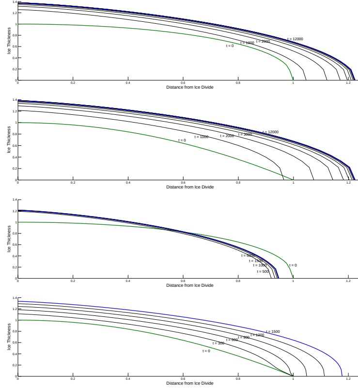
Figure 2: 1D test equations: Ice thickness over the domain evolving from the initial profile (green) to a final steady state profile (blue).
