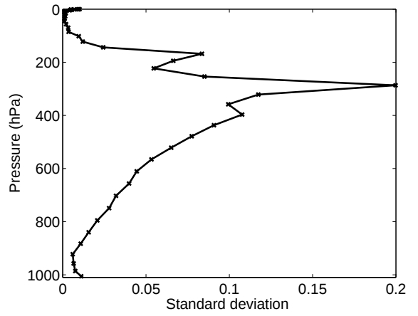
(b) log(Specific humidity) (kg/kg)
