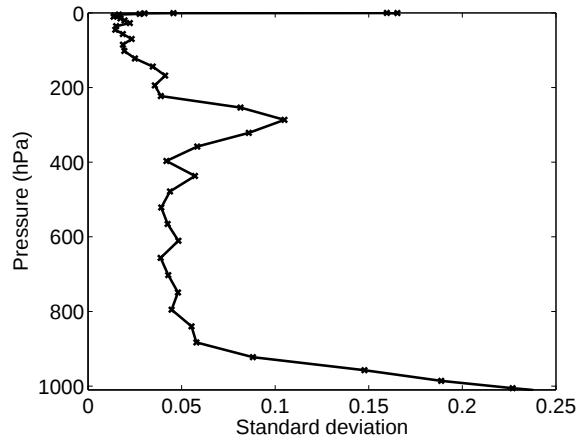
(a) Temperature (K)
