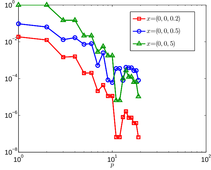
FIGURE 1. Convergence of the absolute error |\text{Var}[u'](\mathbf{x}) - \text{Var}[u'_p](\mathbf{x})| for three points \mathbf{x} inside and outside the unit sphere with respect to the order of the hyperbolic cross p .
