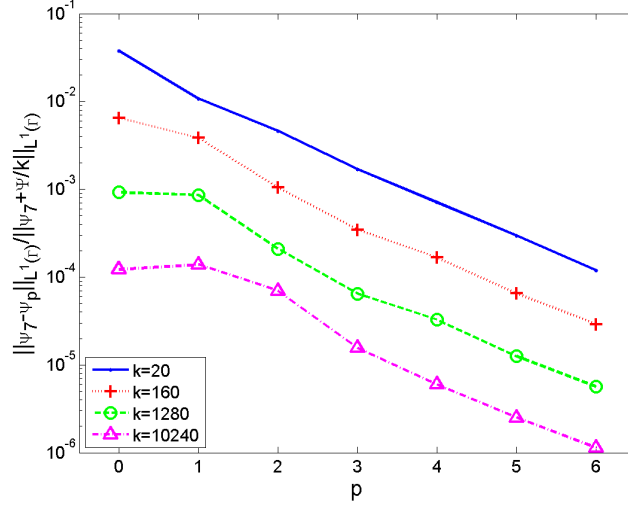
Figure 4: Relative errors in our approximation to \frac{1}{k}[\partial_\nu u] , scattering by a screen
