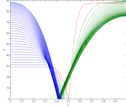
Figure 7: Result of competition model at t = 3.5 , considering the effect of an increased diffusion rate for species 2. Here we use \delta_1 = 0.01, \delta_2 = 0.05 , k_1 = k_2 = 100 , r_1 = r_2 = 1 and \mu = 3 . We run the model with a time step of 0.0001 for 35000 steps, and plot the results every 0.1. We observe that species 2 is able to make initial territorial gains due to its high diffusion rate, even though the competition rate is unaltered.
