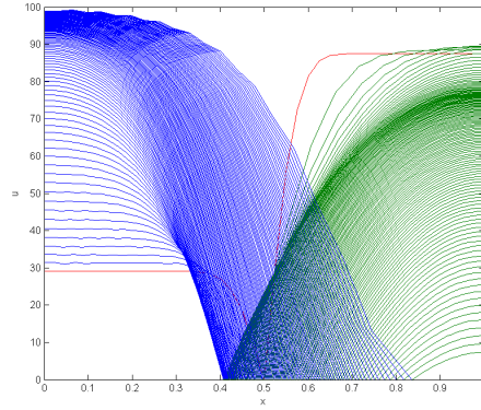
Figure 8: Result of competition model at t = 12.3 , considering the effect of an increased diffusion rate for species 2. Here we use \delta_1 = 0.01, \delta_2 = 0.05 , k_1 = k_2 = 100 , r_1 = r_2 = 1 and \mu = 3 . We run the model with a time step of 0.0001 for 123000 iterations, and plot the results every 0.1. We see that the initial diffusion-driven gains by species 2 are reversed, and that the overall growth characteristics are dominating so that species 1 is gaining territory.
